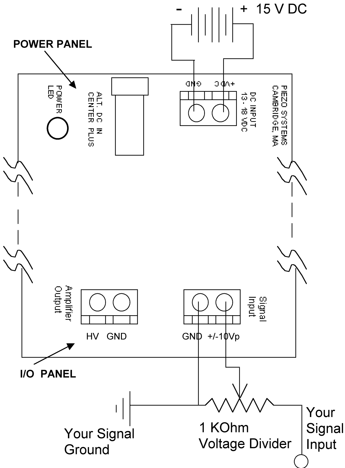
WIRING THE EPA-007 FOR VARIABLE GAIN
